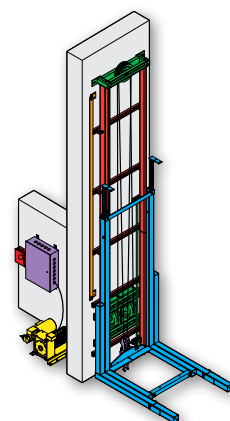
Paca-Lift, Winding Drum Series 118 Capacity 1,000 lbs
